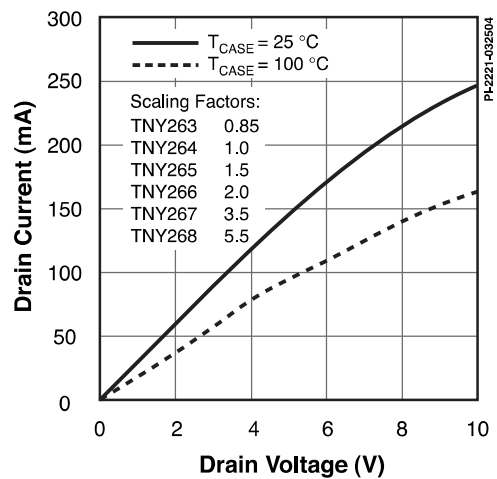
Figure 27. Output Characteristic.
