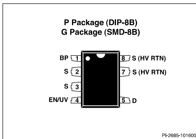
Figure 3. Pin Configuration.
