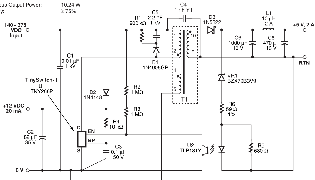
Figure 15. 10 W Standby Supply.
