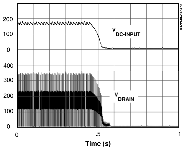
Figure 12. Normal Power-down Timing (without UV).
