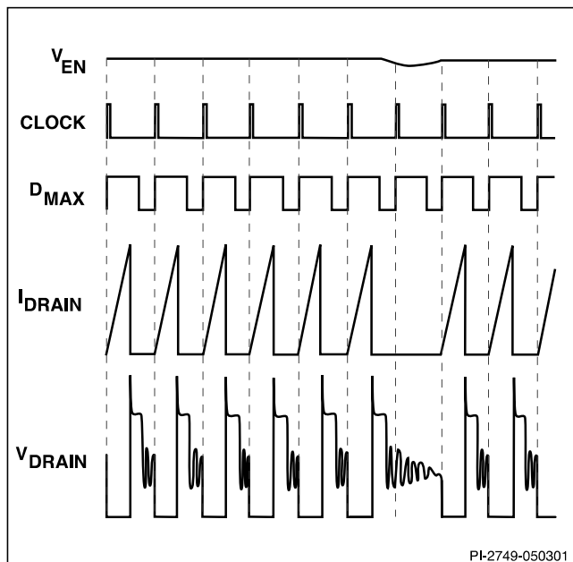
Figure 6. TinySwitch-II Operation at Near Maximum Loading.
