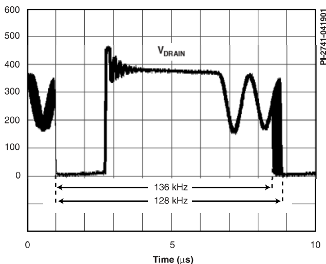
Figure 4. Frequency Jitter.
